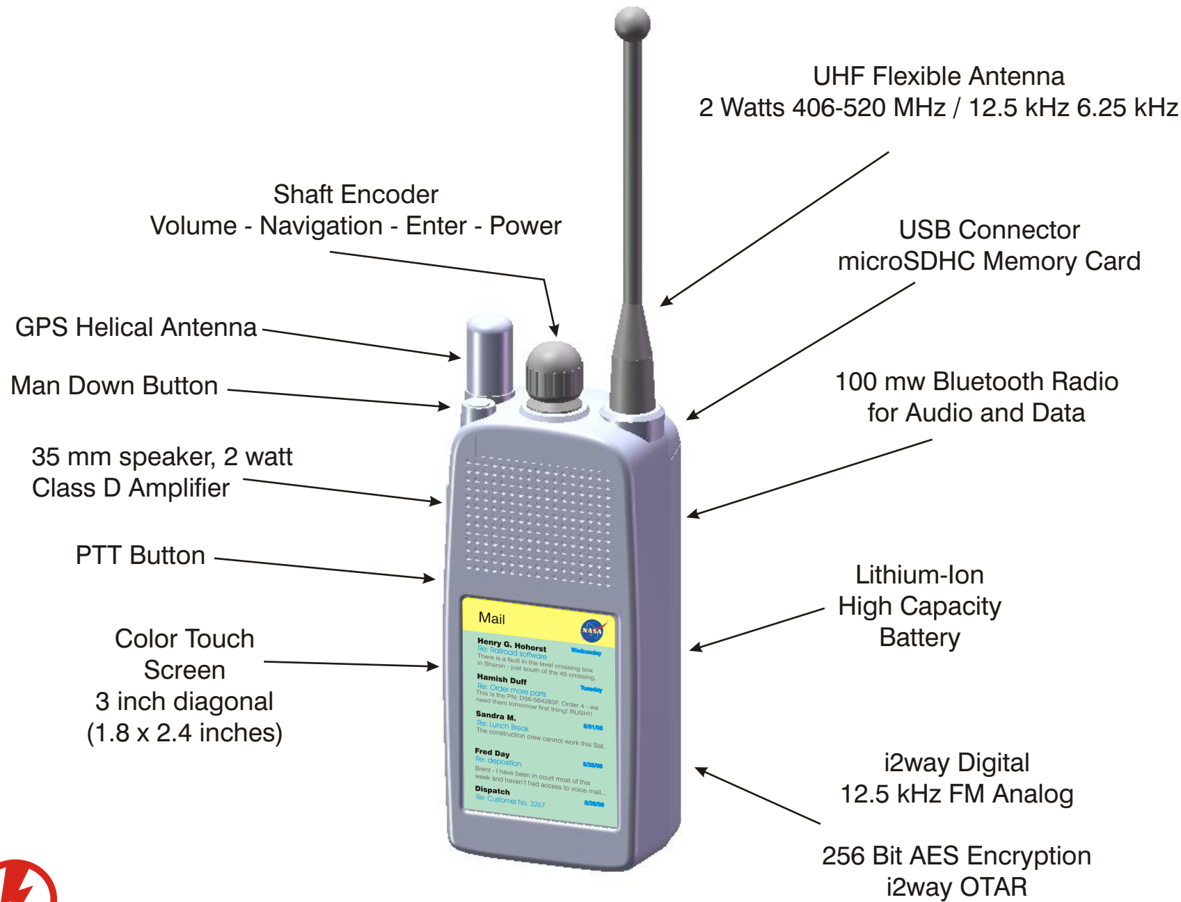
DP-2000 i2way Radio
